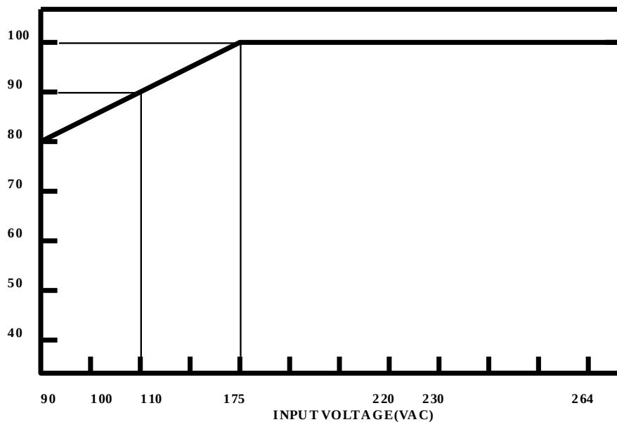
Output Derating VS Input Voltage
